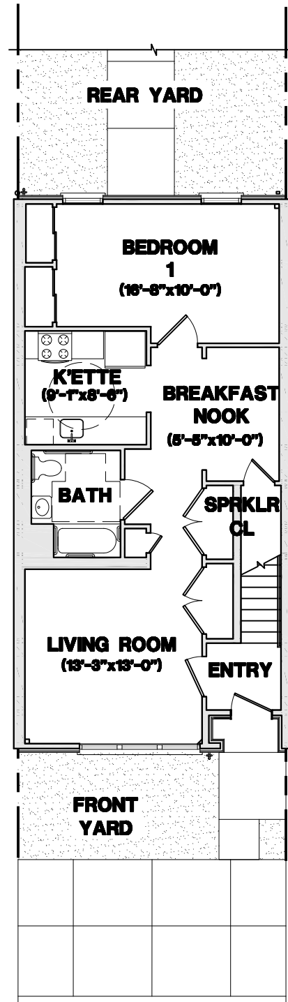
1st FLOOR
